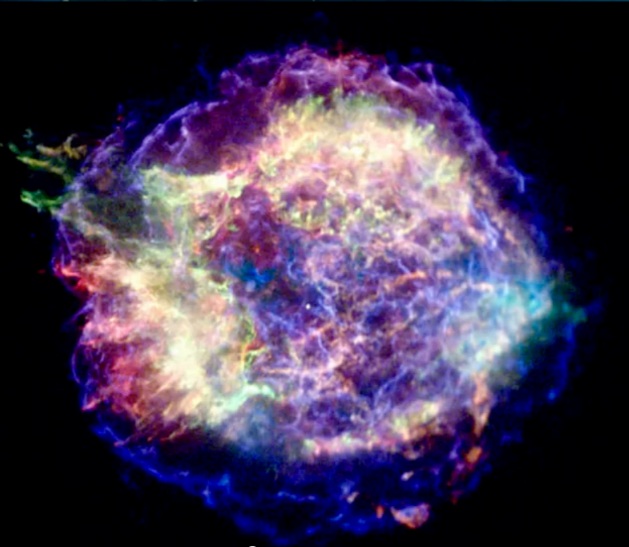
Massive Stars
